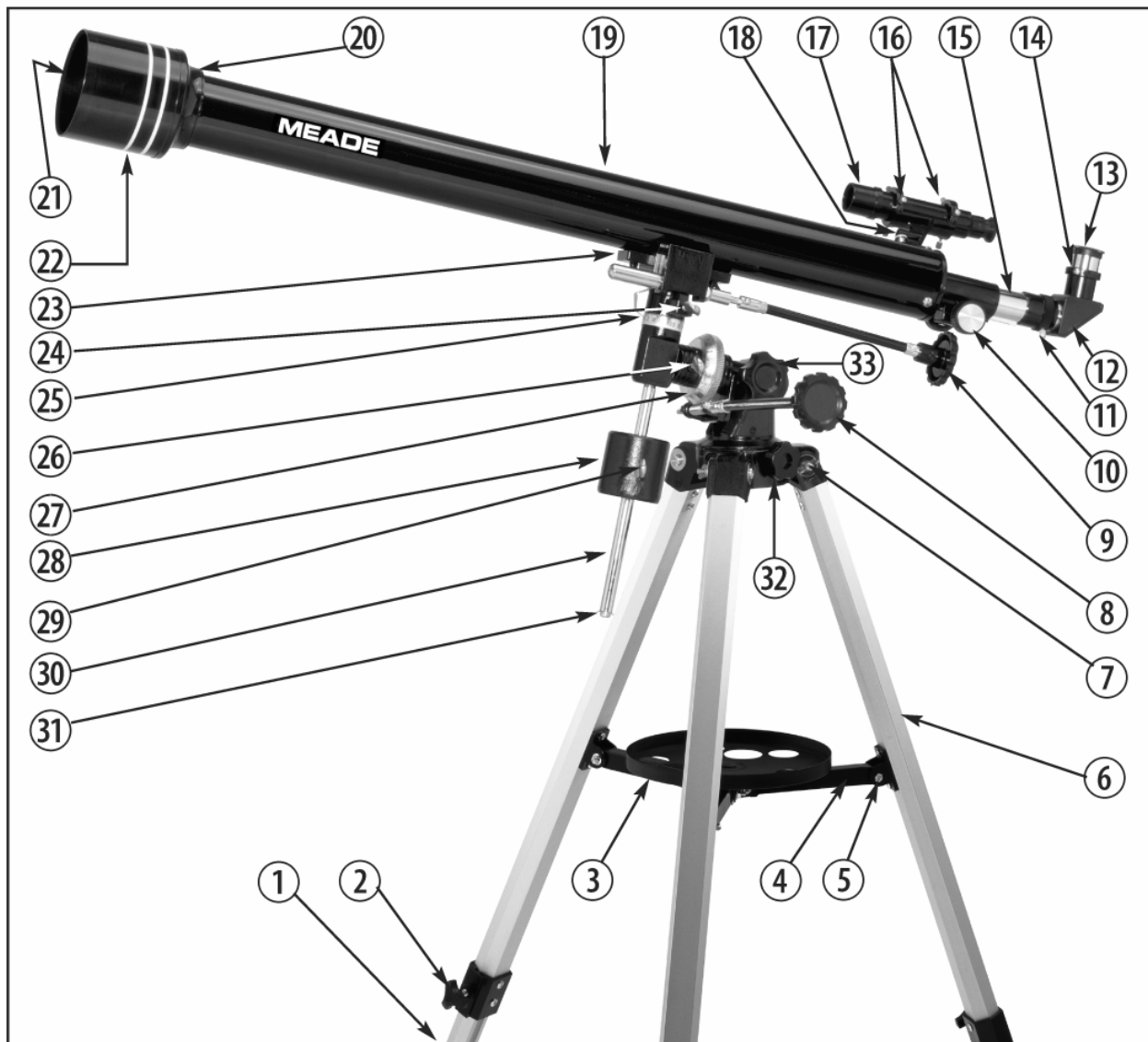
FIGURA 1: Meade 60EQ-A: TELESCOPIO REFRACTOR ECUATORIAL
